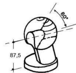
Art. 35-00014 Sfera con asola DX D.85 Raw ball D.85 with oval eyelet - right (Kg.3,015)
