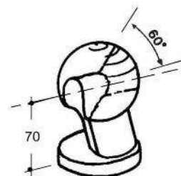
Art. 35-00003 Sfera con asola DX D.60 Raw ball D.60 with oval eyelet - right (Kg.1,122)
