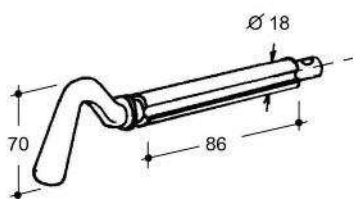
Art. 35-00004 Spinotto a 1 gola D.18 Single fluted locking pin D.18 (Kg.0,301)
