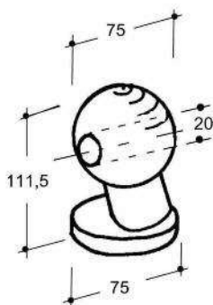
Art. 35-00010 Sfera con foro D.75 Raw ball D.75 with eyelet (Kg.2,160)
