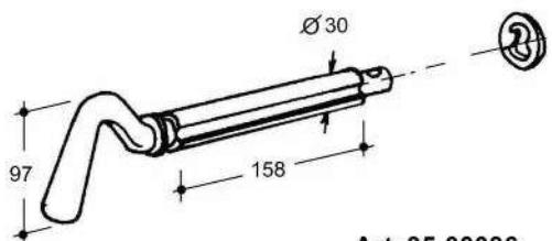
Art. 35-00036 Piastrina a 2 gole Twin fluted raw plate
