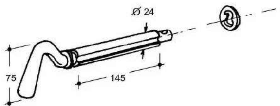
Art. 35-00018 Piastrina a 2 gole Twin fluted raw plate (Kg.0,026)
