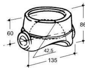
Art. 35-00012 Supporto a sfera D.85 Raw socket for ball D.85 (Kg.3,388)
