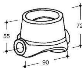
Art. 35-00001 Supporto a sfera D.60 Raw socket for ball D.60 (Kg.1,290)
