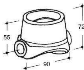
Art. 35-00000 Supporto a sfera D.60 forgiato Raw socket for ball D.60 forged (Kg.1,290)
