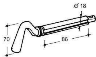
Art. 35-00006 Spinotto a 2 gole D.18 Twin fluted locking pin D.18 (Kg.0,302)
