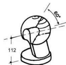
Art. 35-00032 Sfera con asola DX D.110 Raw ball d. 110 with oval eyelet - right (Kg.7,536)
