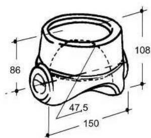
Art. 35-00020 Supporto a sfera D.95 Raw socket for ball D.95 (Kg.5,630)
