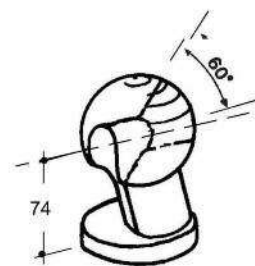
Art. 35-00011 Sfera con asola DX D.75 Raw ball D.75 with oval eyelet - right (Kg.1,900)
