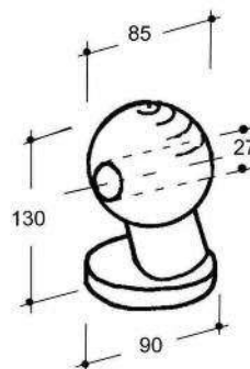
Art. 35-00013 Sfera con foro D.85 Raw ball D.85 with eyelet (Kg.3,336)
