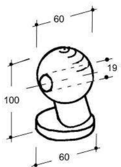
Art. 35-00000/1 Sfera con foro Ø60 forgiata Raw ball Ø60 with eyelet forged (Kg.1,243)
