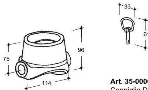
Art. 35-00009 Supporto a sfera D.75 Raw socket for ball D.75 (Kg.2,555)
