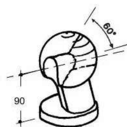
Art. 35-00022 Sfera con asola DX D.95 Raw ball D.95 with oval eyelet - right (Kg.4,630)
