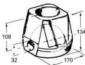
Art. 35-00030 Supporto a sfera D.110 Raw socket for ball D.110 (Kg.9,210)
