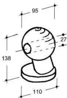
Art. 35-00021 Sfera con foro D.95 Raw ball D.95 with eyelet (Kg.4,810)
