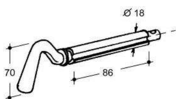
Art. 35-00004 Spinotto a 1 gola D.18 Single fluted locking pin D.18 (Kg.0,301)
