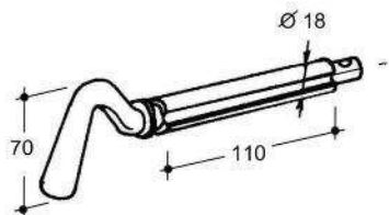
Art. 35-00006/L Spinotto a 2 gole D.18 L=110 Twin fluted locking pin L=110 D.18 (Kg.0,365)
