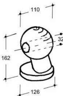
Art. 35-00031 Sfera con foro D.110 Raw ball D.110 with eyelet (Kg.8,165)
