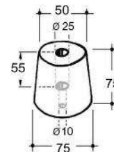
Art. 49-00062 (Kg.0,305) Tampone in gomma D.75xD.50xH.75 Conical rubber buffer D.75xD.50xH.75
