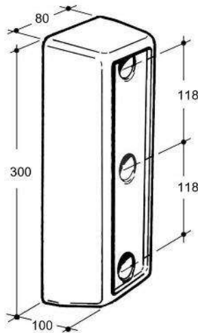
Art. 49-00049 (Kg.2,753) Tampone in gomma 300x80xH.100 Rubber buffer 300x80xH.100
