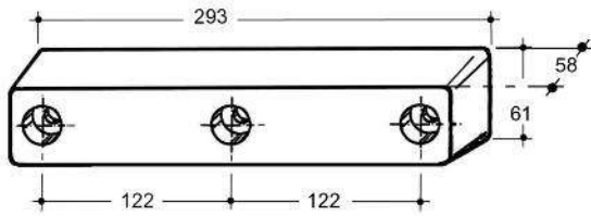
Art. 49-00048 Tampone in gomma 293x61xH.58 Rubber buffer 293x61xH.58
