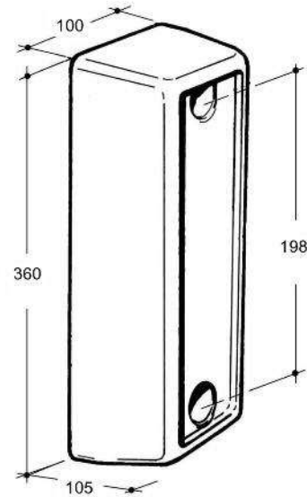
Art. 49-00061 (Kg.4,034) Tampone in gomma 360x100xH.105 Rubber buffer 360x100xH.105
