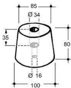
Art. 49-00050 (Kg.0,655) Tampone in gomma D.100xD.85xH.80 Conical rubber buffer D.100xD.85xH.80
