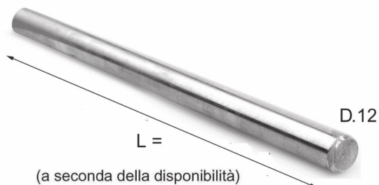
Art. 31-00011 (Kg/ml. 2,670) Tondino inox trafilato L=3000 o L=4000 D.12 Full-drawn steel round bar L=3000 / L=4000 D.12
