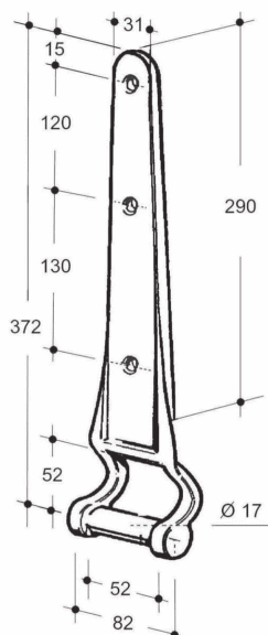
Art. 31-00155 Cerniera ribaltabile alta zinc.H.372 Galv.high hinge for dump trucks H.372 (Kg.1,075)
