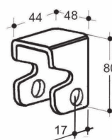
Art. 31-00046 Supporto cern. (foro D.21) Raw support (hole D.21) (Kg.0,244)
