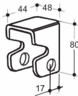
Art. 31-00046 Supporto cern. (foro D.21) Raw support (hole D.21) (Kg.0,244)
