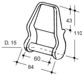
Art. 31-00180 Cern.doppia apert. piccola L=110 Double opening light hinge L=110 (Kg.0,550)
