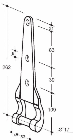
Art. 31-00045 Cern.ribaltabile alta zinc.H.262 Galv.high hinge for dump trucks H.262 (Kg.0,765)
