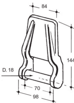
Art. 31-00186 Cern. doppia apertura L=144 Double opening hinge L=144 (Kg.1,118)
