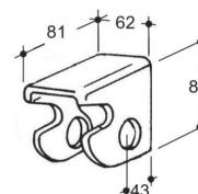
Art. 31-00187 Supporto cerniera foro D.26 Hinge support hole D.26 (Kg.0,597)
