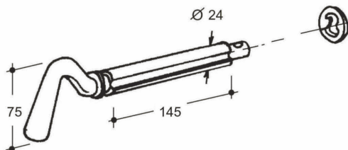
Art. 35-00018 Piastrina a 2 gole Twin fluted raw plate (Kg.0,026)
