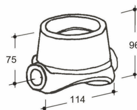
Art. 35-00009 Supporto a sfera D.75 Raw socket for ball D.75 (Kg.2,555)
