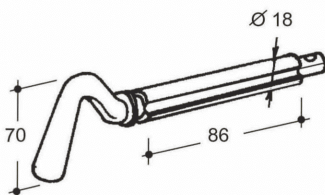
Art. 35-00006 Spinotto a 2 gole D.18 Twin fluted locking pin D.18 (Kg.0,302)
