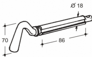
Art. 35-00004 Spinotto a 1 gola D.18 Single fluted locking pin D.18 (Kg.0,301)
