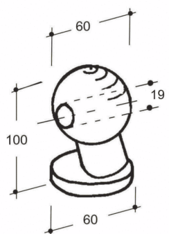
Art. 35-00000/1 Sfera con foro Ø60 forgiata Raw ball Ø60 with eyelet forged (Kg.1,243)
