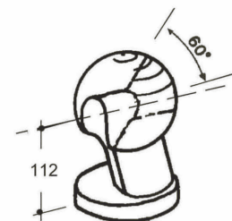
Art. 35-00032 Sfera con asola DX D.110 Raw ball d. 110 with oval eyelet - right (Kg.7,536)
