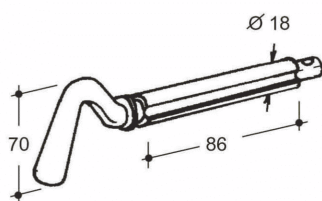
Art. 35-00004 Spinotto a 1 gola D.18 Single fluted locking pin D.18 (Kg.0,301)
