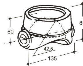
Art. 35-00012 Supporto a sfera D.85 Raw socket for ball D.85 (Kg.3,388)
