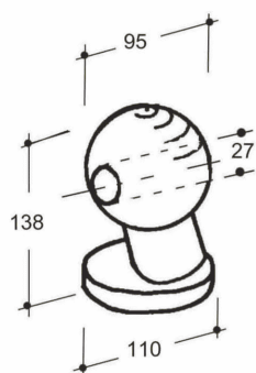
Art. 35-00021 Sfera con foro D.95 Raw ball D.95 with eyelet (Kg.4,810)
