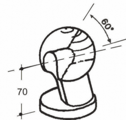
Art. 35-00003 Sfera con asola DX D.60 Raw ball D.60 with oval eyelet - right (Kg.1,122)
